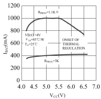
Recharging Current vs Battery Voltage
