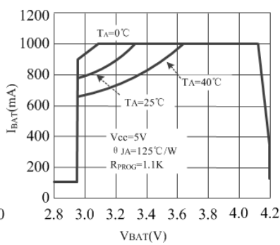
Recharging Current vs Battery Voltage
