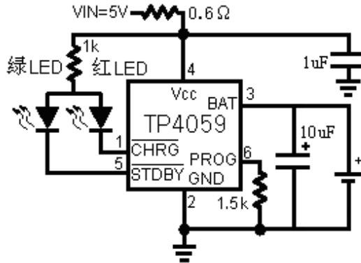
Full function single section lithium battery charger (connected to dissipation resistor)
