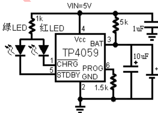
Battery free dual light off single lithium battery charger
