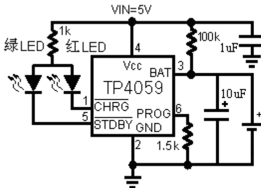
No battery, no flashing light, single lithium battery charger
