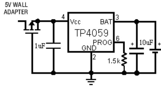
Charger with input reverse polarity protection
