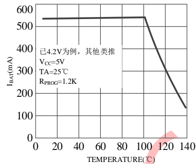
4.2V Charge Current vs Temperature
