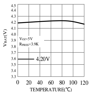
Regulated Output (Float) Voltage vs Temperature
